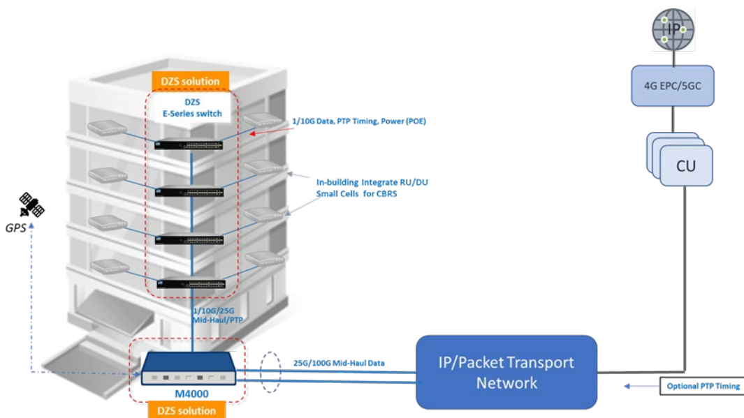
Typical Application: E-Series switch provides Small Cell aggregation while M-Series switch implements Mobile backhaul
